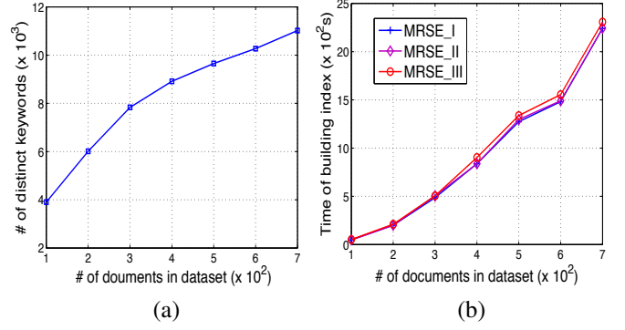
Fig. 3: Relationship between number of documents in dataset and (a) Number of distinct keywords in dataset, and (b) Time cost for building searchable index.
