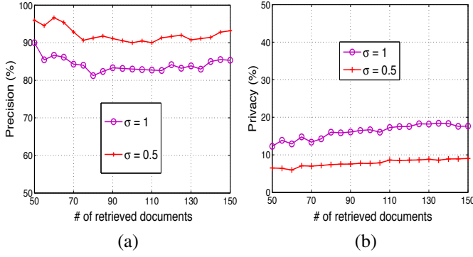
Fig. 2: With different choice of standard deviation \sigma for the random variable \varepsilon , there exists tradeoff between (a) Precision, and (b) Rank Privacy.
