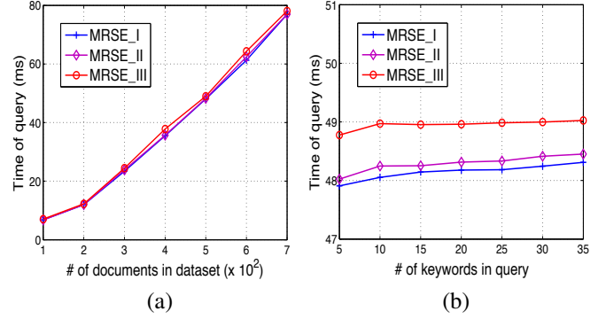
Fig. 5: Time cost of query. (a) For the same number (10) of keywords in a query within different number of documents in dataset. (b) For different number of keywords in a query within the same number (500) of documents in dataset.
