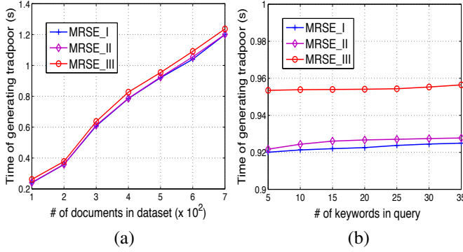
Fig. 4: Time cost of generating trapdoor. (a) For the same number (10) of keywords in a query within different number of documents in dataset. (b) For different number of keywords in a query within same number (500) of documents in dataset.
